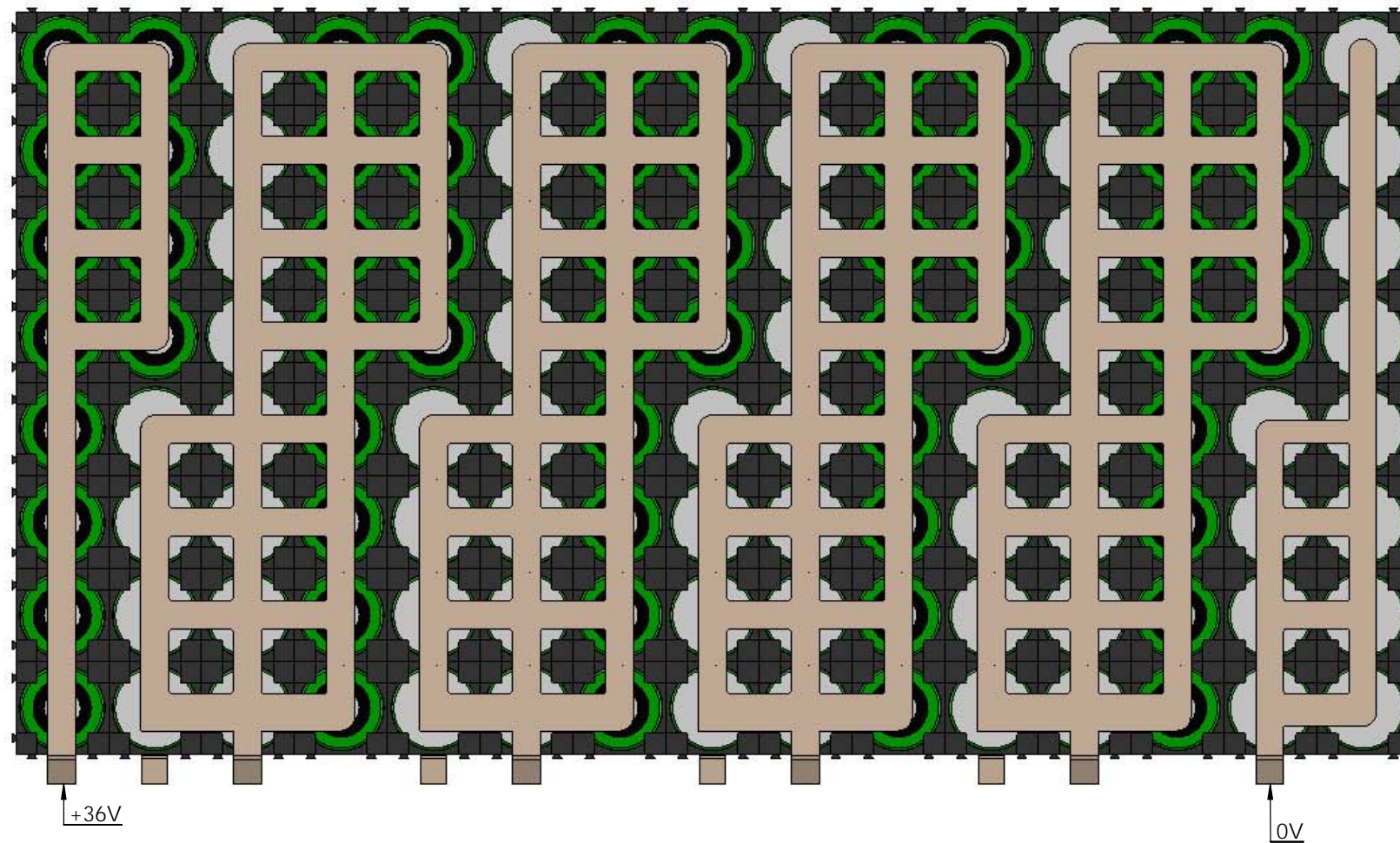
BATTERY PACK TOP VIEW
